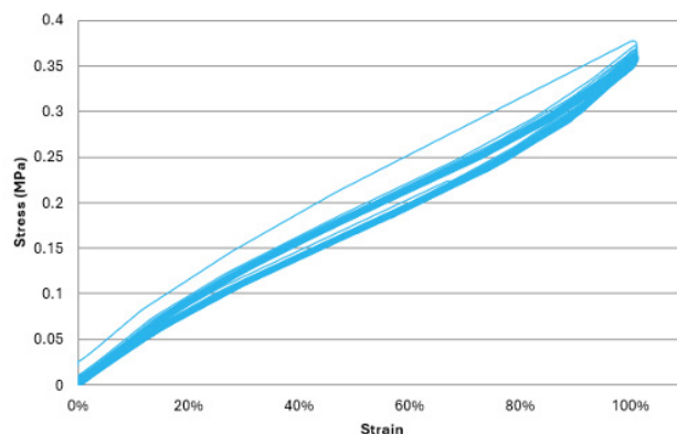
P3 Silicone 25A, 100% extension, 100 mm/min, 50 cycles
