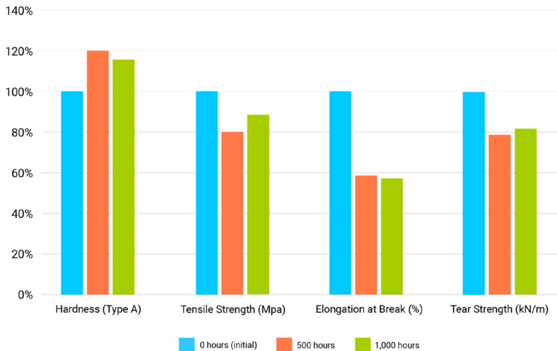
Mechanical Properties After Aging in 150 °C After 500 & 1,000 hours
